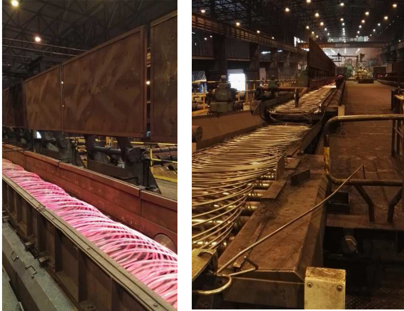
Figure 8: Wire Rod Mill . Zone 1 and Zone 2
